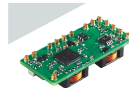
Point of Load DC/DC Converters DOSA / POLA Current Range: 0~60A
